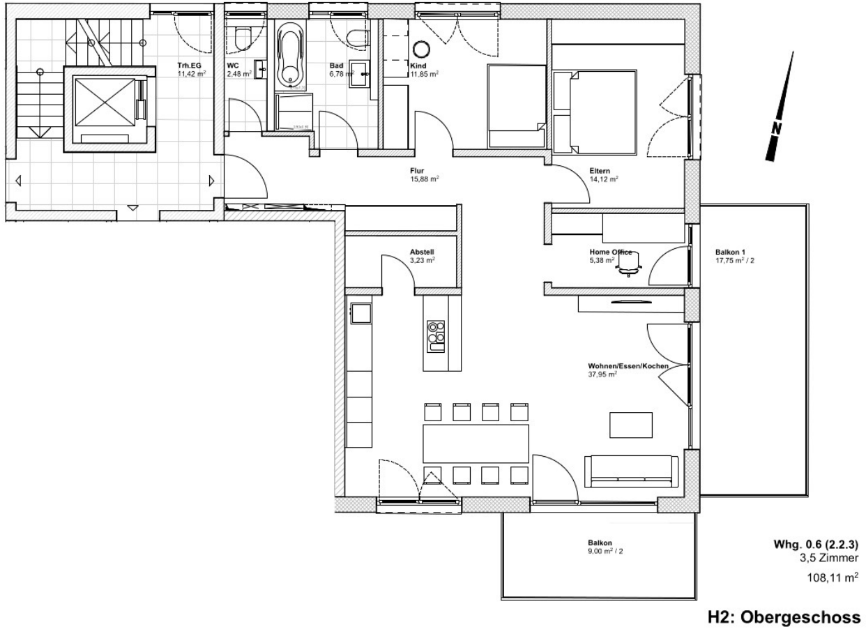
Grundriss Whg. 2.2.3
